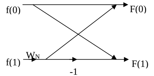
Fig(c): FFT Butterfly for 2-point DFT.
